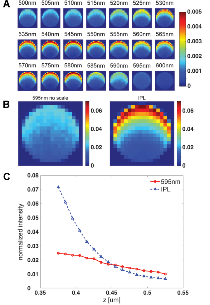
Fig. 4. (A) Normalized absorbed energy distribution within 0.081 \mu m radius vessel over 500–600 nm wavelength range at 5 nm increments. All energy distribution maps are plotted on the same color scale. (B) Comparison of 595 nm normalized absorbed energy distribution and composite narrowband IPL 500–60 nm energy distribution of 0.081 \mu m radius vessel. The average absorbed energy in the upper half of the line profile of the IPL is 0.0406 \pm 0.0004 while the average in the lower half is 0.0098 \pm 0.0003. At 595 nm the average absorbed energy in the upper half is 0.0216 \pm 0.0004 and in the lower half is 0.0131 \pm 0.0003. Composite vessel indicates that most absorbed energy is contained within the top half of the vessel, while the bottom half has lower absorbed energy compared to 595 nm. (C) Line profile of normalized absorbed energy distribution with one-sigma error bars (bars are smaller than symbol) using 595 nm and narrowband IPL irradiation. With the former, the average absorbed energy is more evenly distributed over the entire vessel, as compared to the narrowband IPL absorbed energy.
